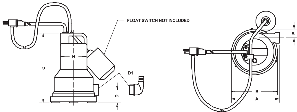
Fig. 38 Dimensional drawings
