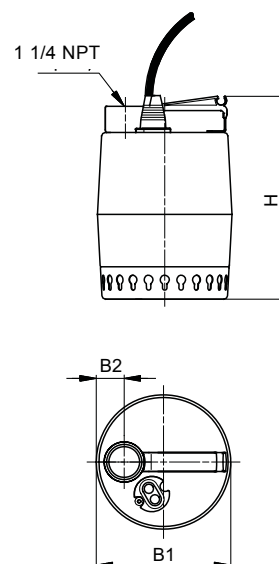
Fig. 10 Pump dimensions
