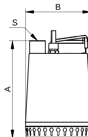
Fig. 14 Pump dimensions
