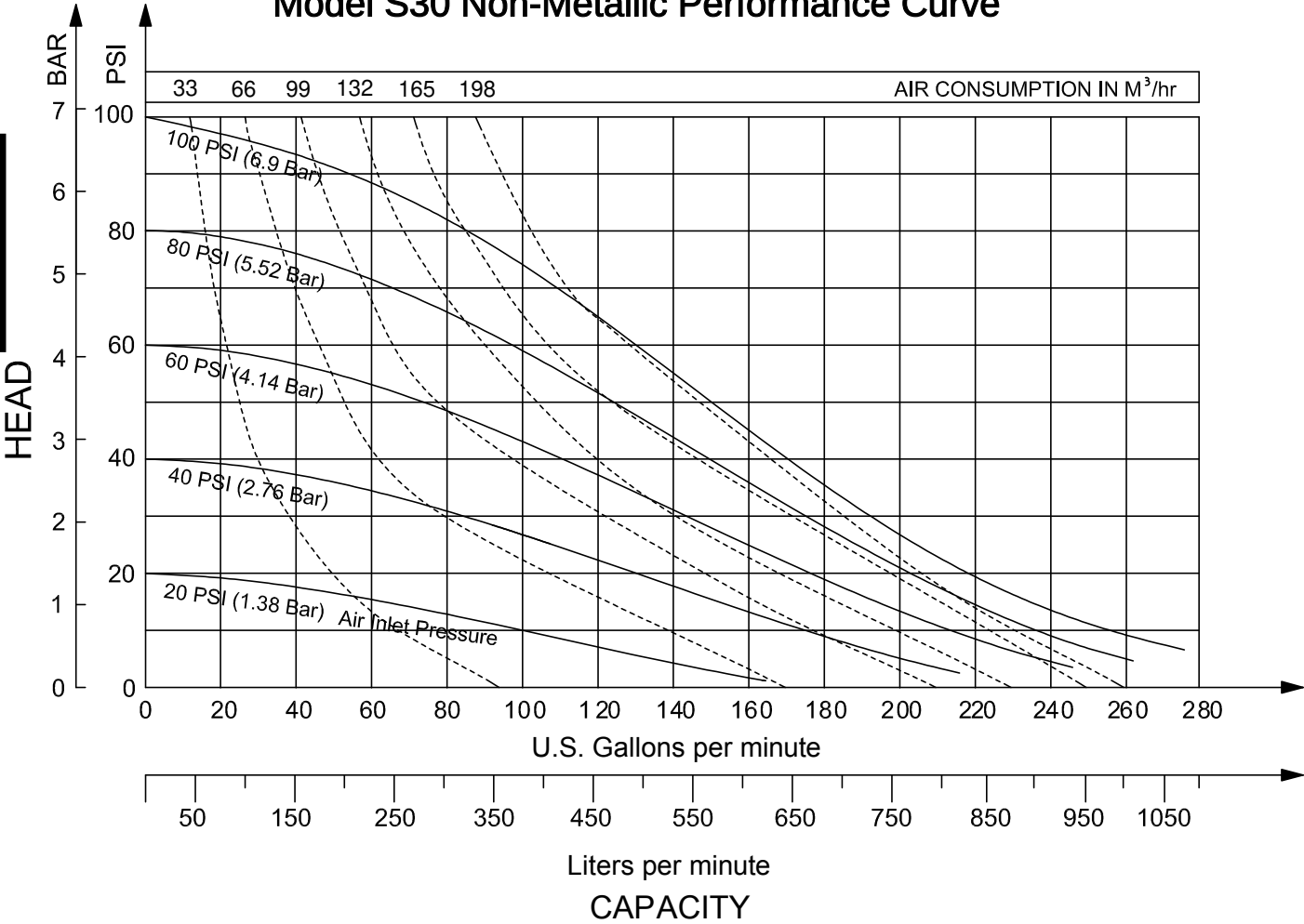
Model S30 Non-Metallic Performance Curve
