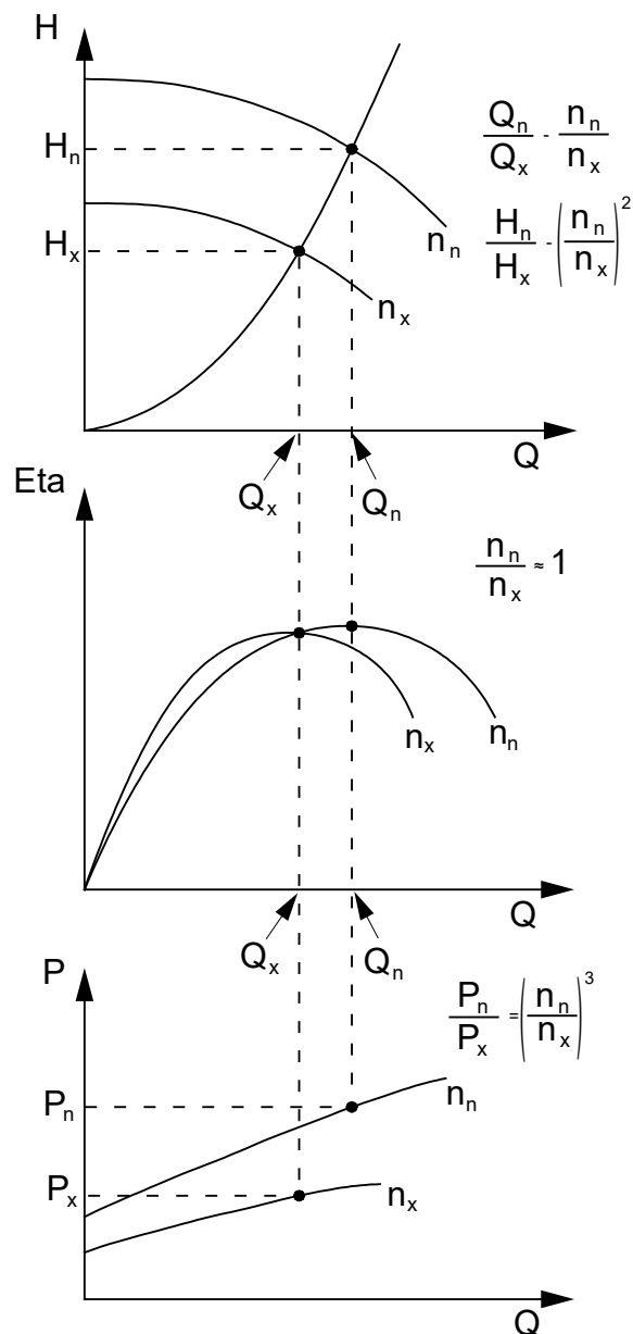
Affinity equations
