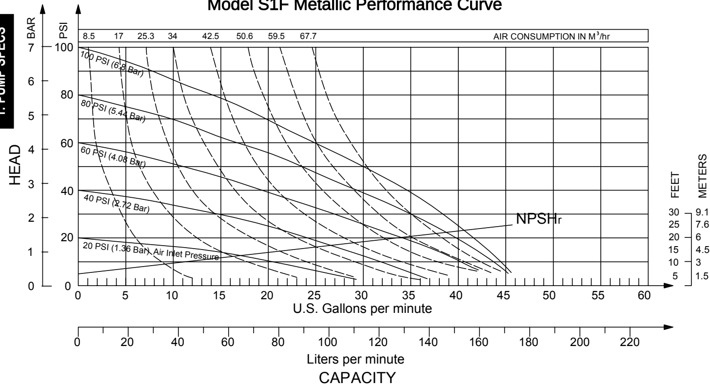
Model S1F Metallic Performance Curve
