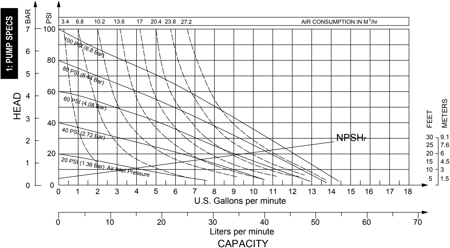
Model S05 Non-Metallic Performance Curve
